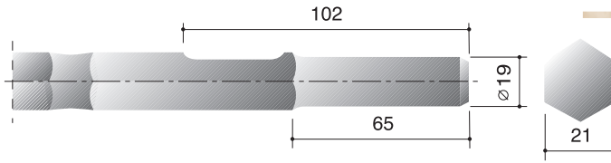
Shank: Ø 19x65 / 21mm
