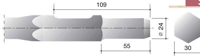
Shank: Ø 24x55 / 30mm
