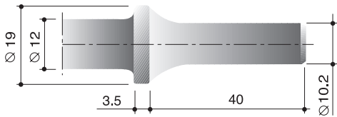
Shank: \varnothing 10.20(0.401") \times 40\text{mm} Taper Shank.
